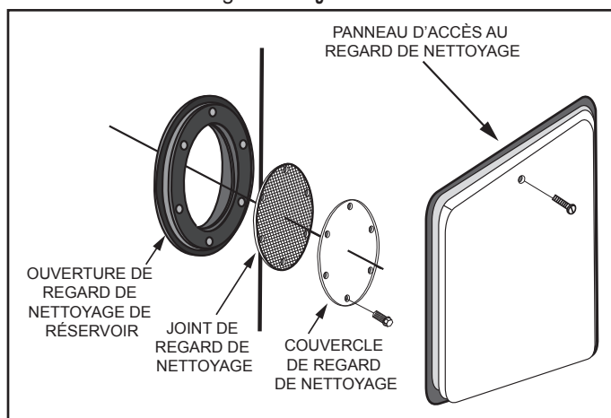
Figure 61. Regard de nettoyage
