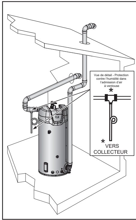
Figure 43. Ventouse, évacuation verticale, admission horizontale
