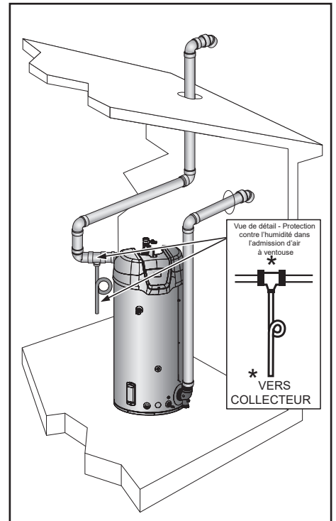
Figure 44. Ventouse, évacuation horizontale, admission verticale
