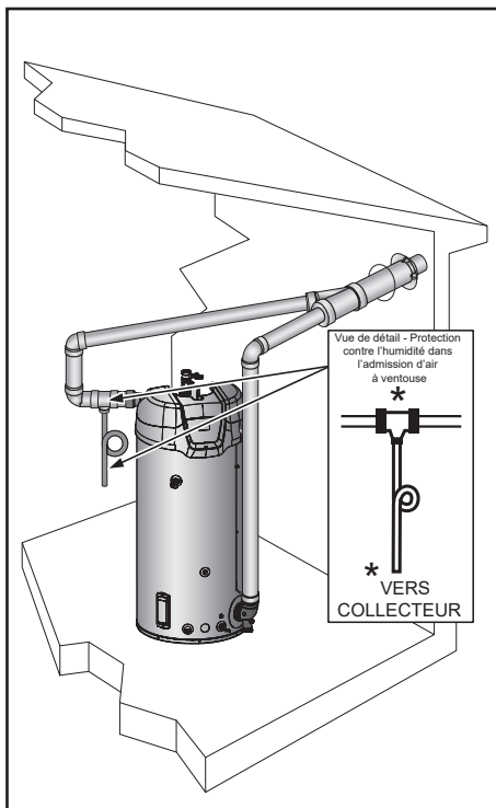
Figure 46. Ventouse concentrique horizontale
