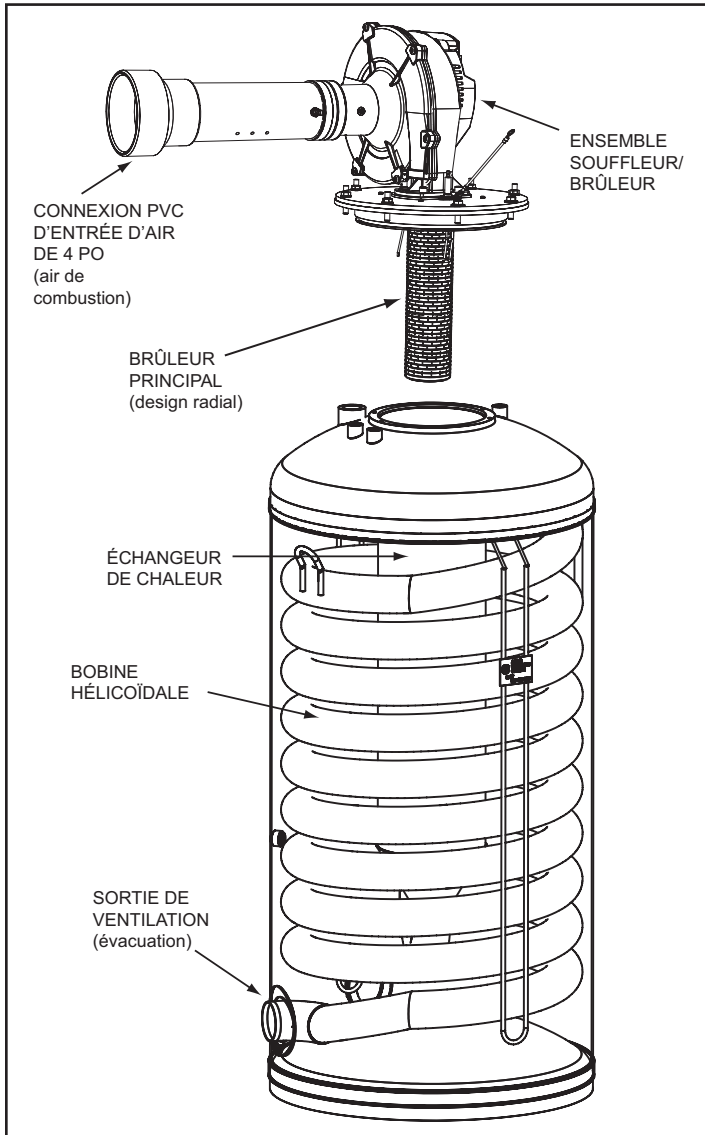
Figure 1. Composants du chauffe-eau
