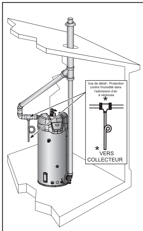
Figure 45. Ventouse concentrique verticale
