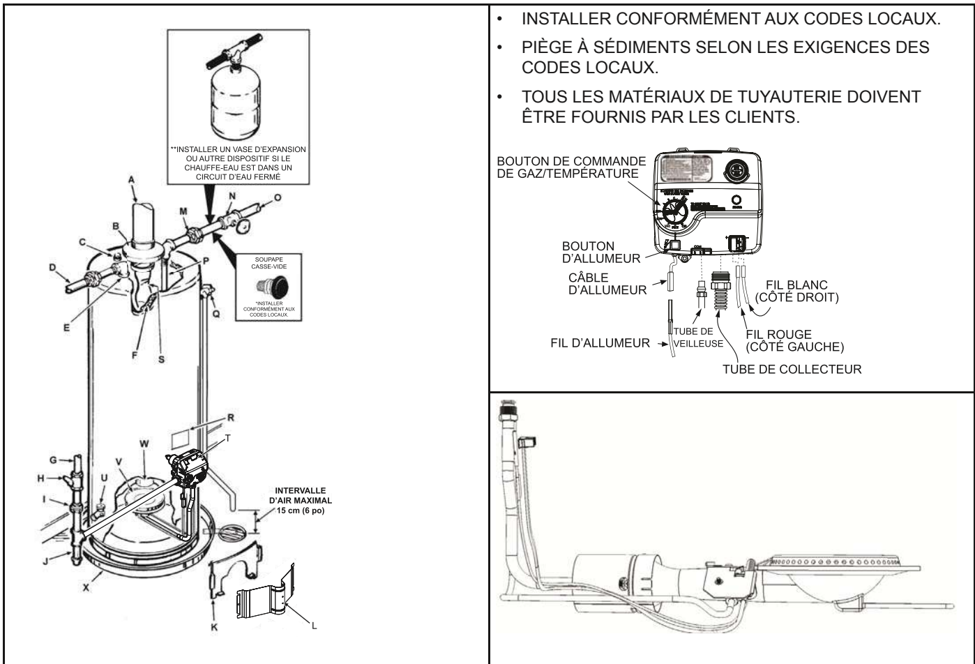
FIGURE 1. INSTALLATION TYPIQUE
