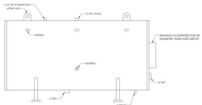
Figure 5-2_Horizontal Tank
