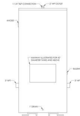
Figure 5-1_Vertical Tank
