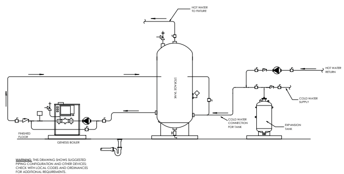
Figure 2-2_Vertical Tank Piping Diagram, Non-Condensing
