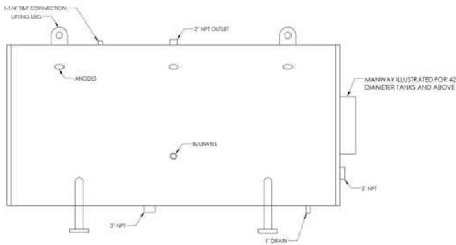
Figure 5-3 _Horizontal Storage Tank w/Anodes
