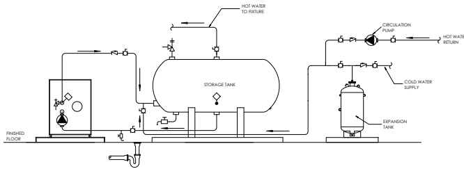
Figure 2-3_Horizontal Tank Piping Diagram - Non-Condensing
