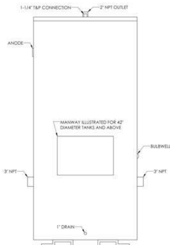
Figure 5-4 _Vertical Storage Tank w/Anodes
