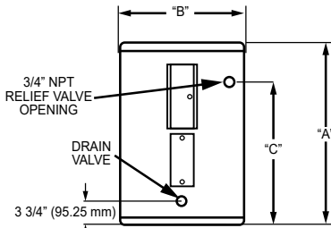
FRONT VIEW DELC 30/40/50 DENC 30/40
