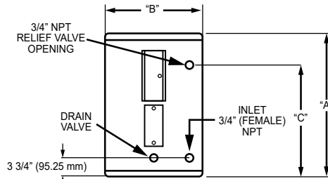
FRONT VIEW DEJC 50/66
