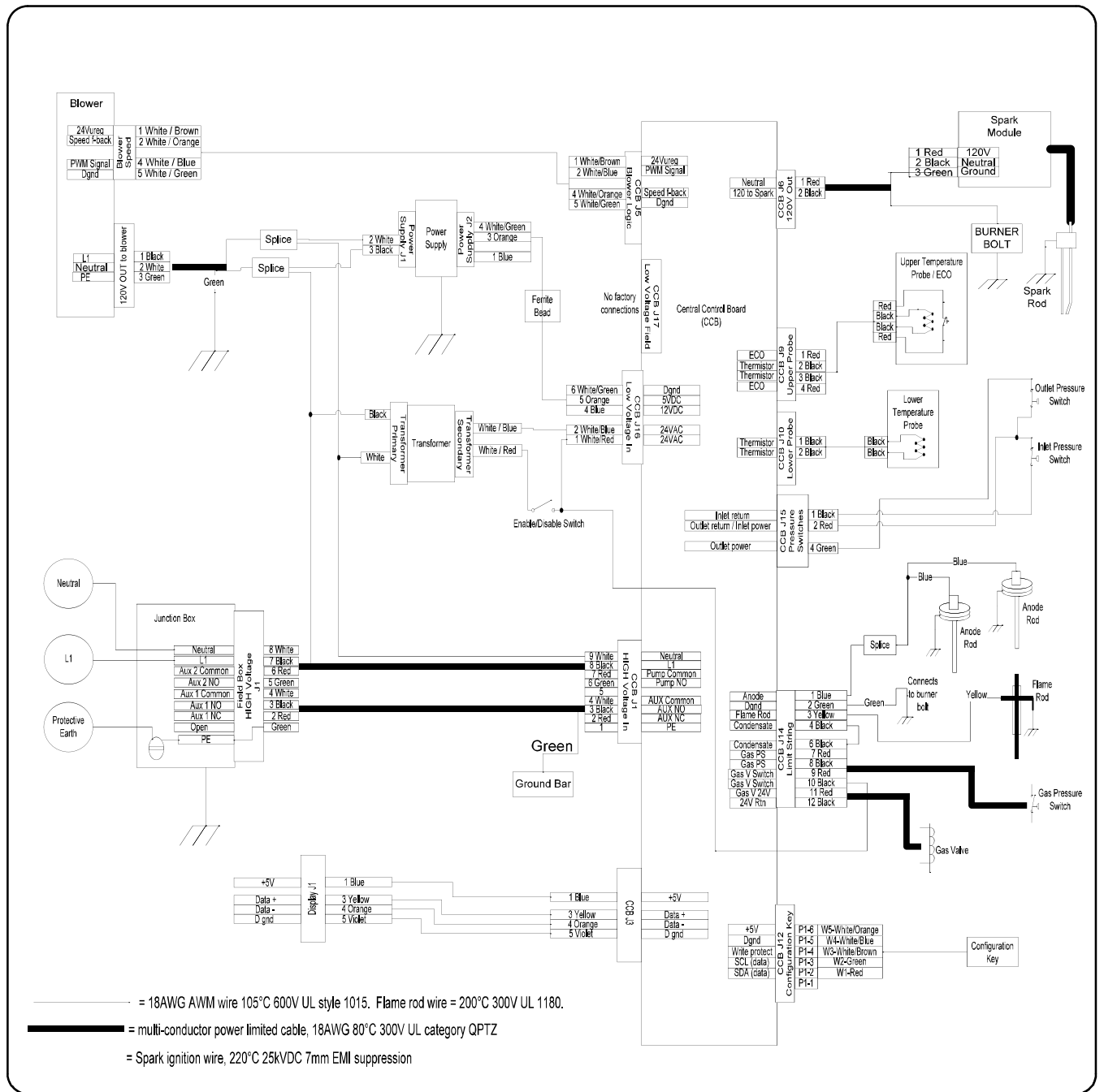
Figure 67. Wiring Diagram
