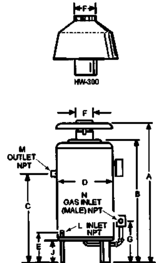
FIGURE 1. DIMENSIONS
